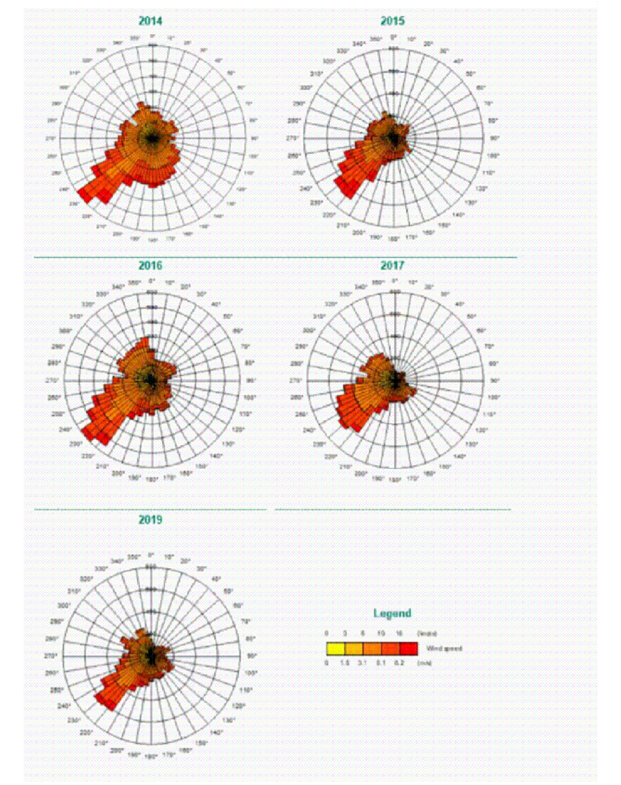
WIND ROSE STUDY FOR STANSTED AIRPORT
